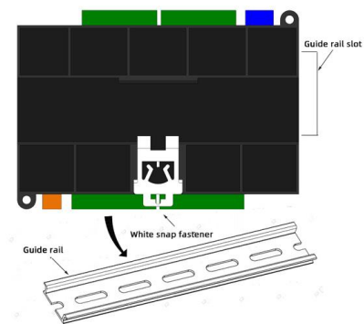
Figure 4: Pull down the white snap of the product and insert it into the rail strip. Then press the white snap upwards as shown in the figure to fix it.
